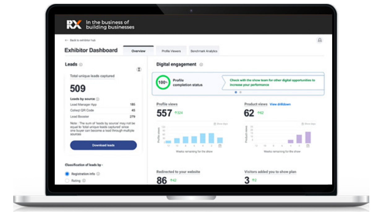
DASHBOARD
